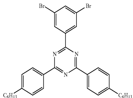
Comparative Monomer 1
