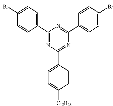
Comparative Monomer 2
